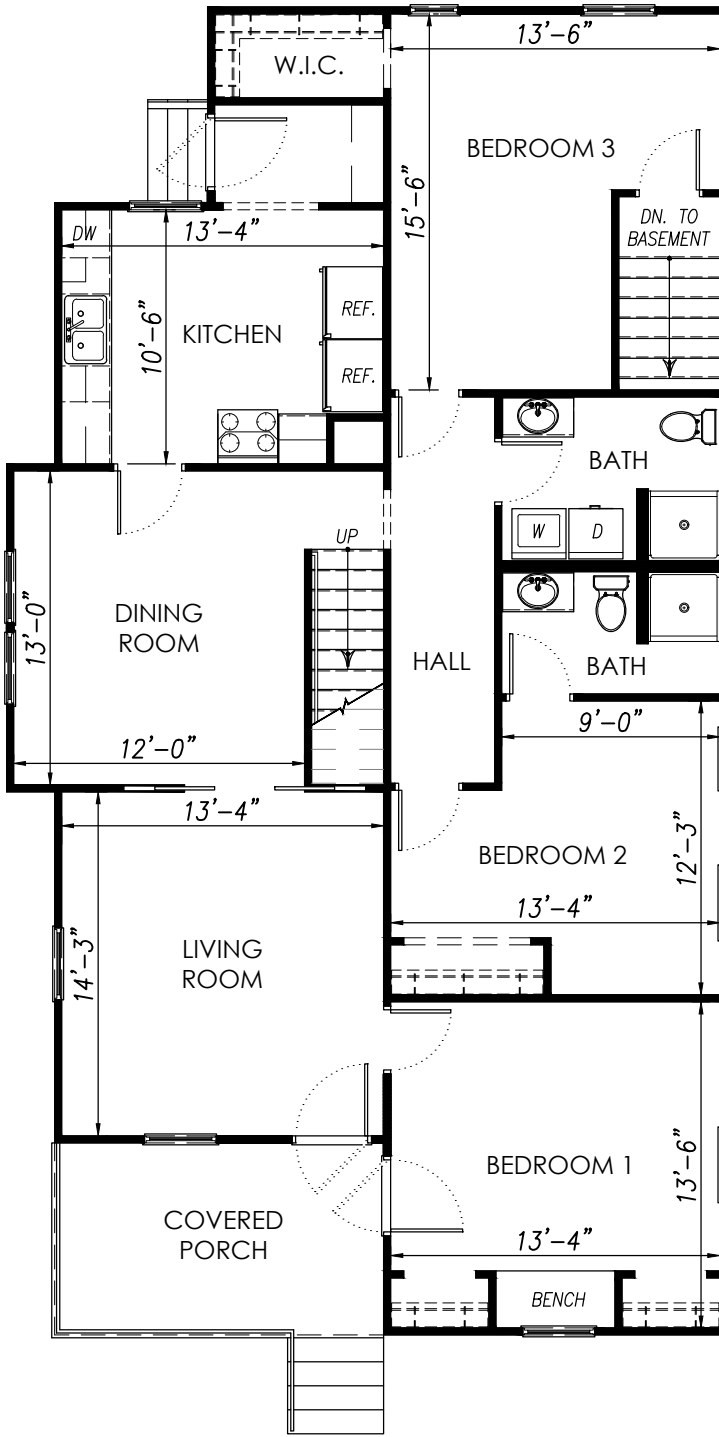
FIRST FLOOR
