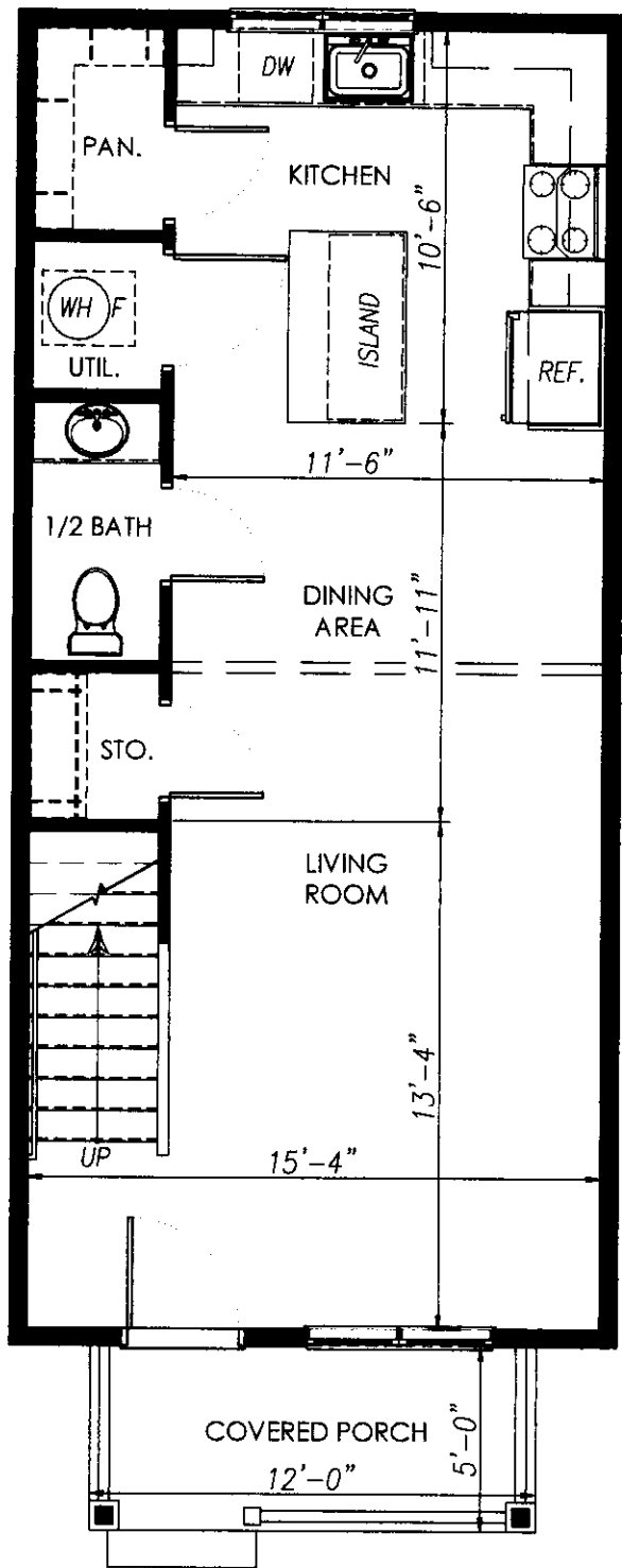
FIRST FLOOR
