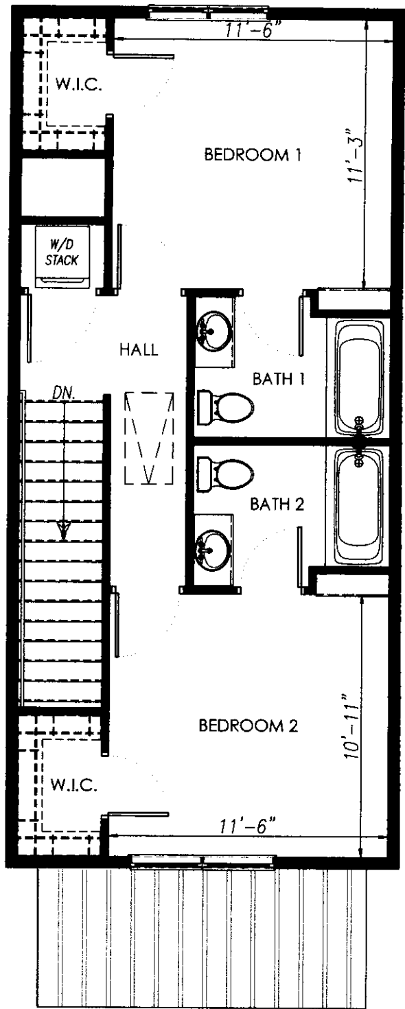
SECOND FLOOR
