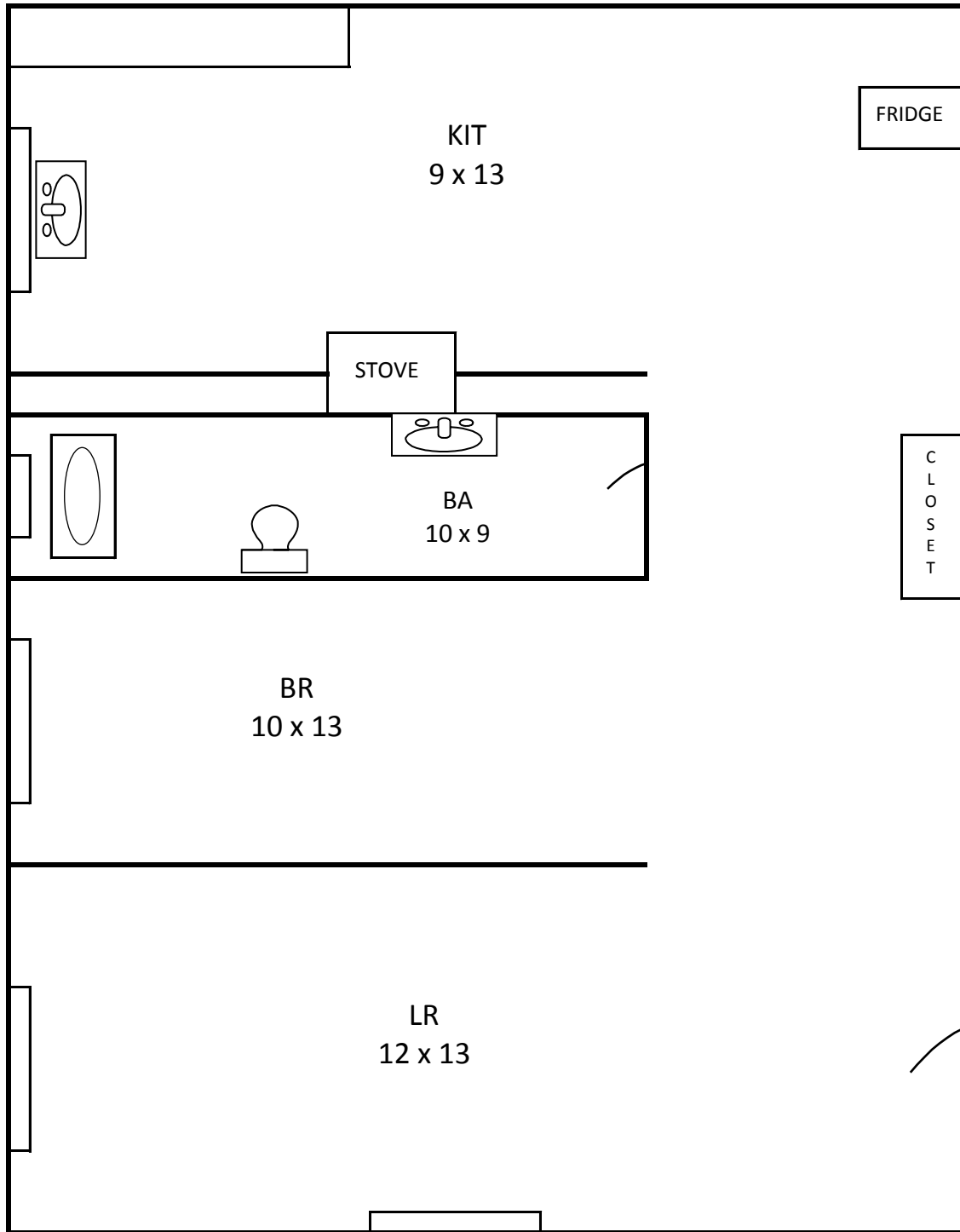
Cambridge III - 1 Bedroom Layout 714 E. Atwater - Apt. 1F 650 Square Feet
