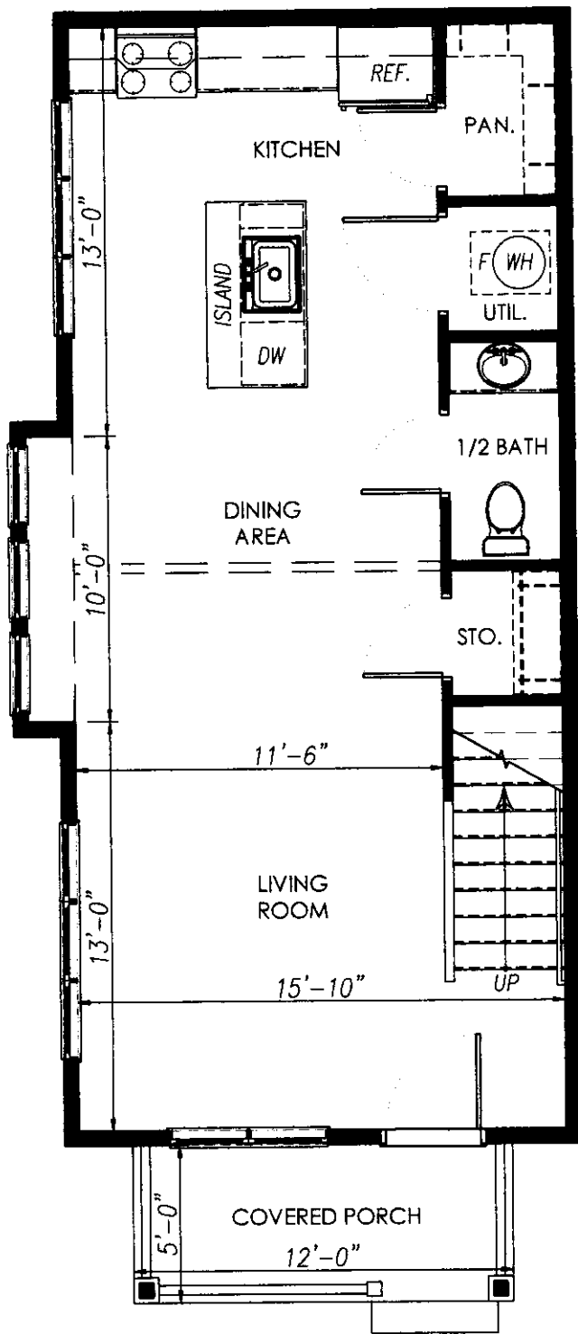
FIRST FLOOR
