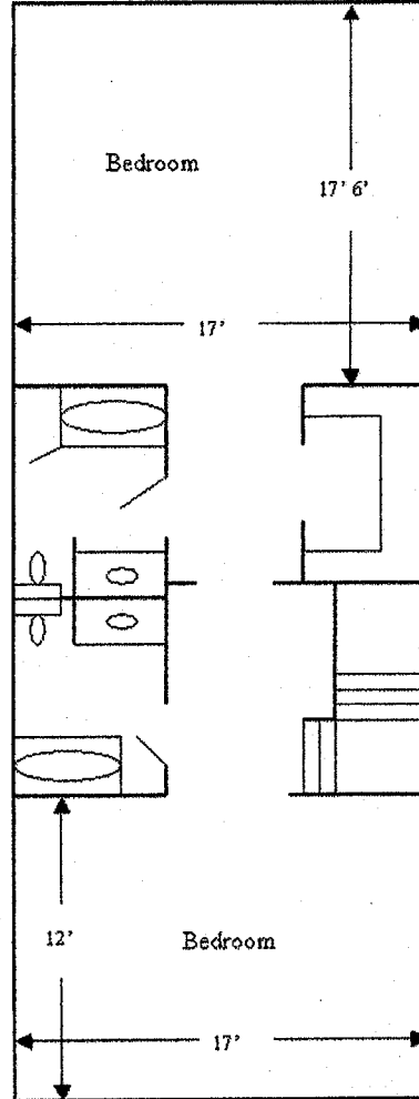
The Gables - C - E 2 Bedroom Layout 1720 Square Feet
